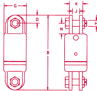
S-2 Jaw & Jaw
