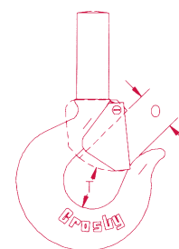
Shank Hook dimension with PL Latch Assembled
