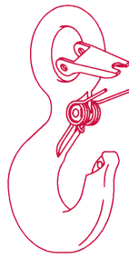
Figure 5: IMPORTANT – Instructions for Assembling S-4320 Latch on Crosby 320N Hooks
