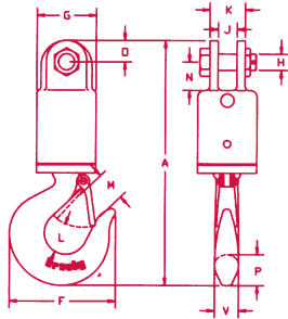
S-1 Jaw & Hook
